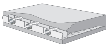
Cliprail (screeded floor on sub base)
