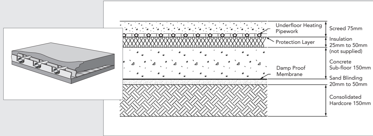
Screeded Floor on Sub Base (Insulation not supplied)
