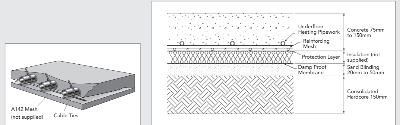
Mesh System (Concrete floor structure shown)
