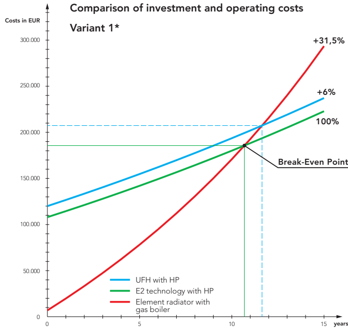
Heat pump versus gas boiler adaptation/steel elements. Investment and operating costs over a period of 15 years
