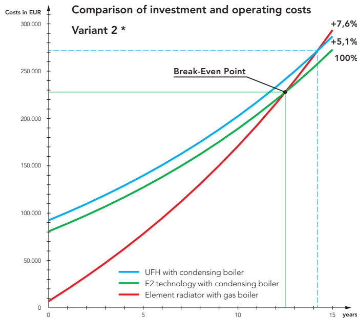
Condensing boiler versus gas boiler adaptation/steel elements. Investment and operating costs over a period of 15 years.
