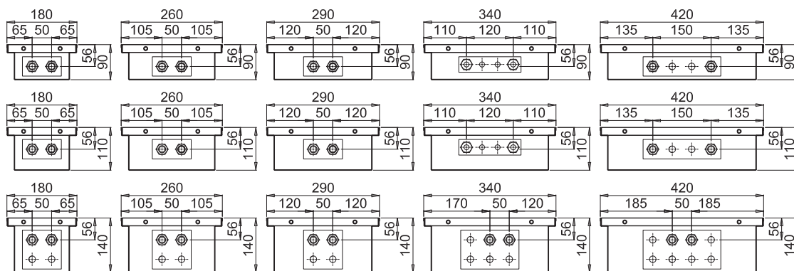
Connection from the left
