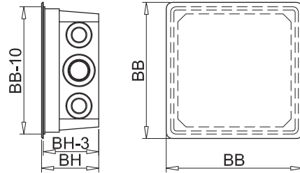
Flush-mounted version
