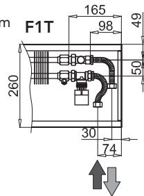
structure width 260 mm structure height 90, 140 mm
