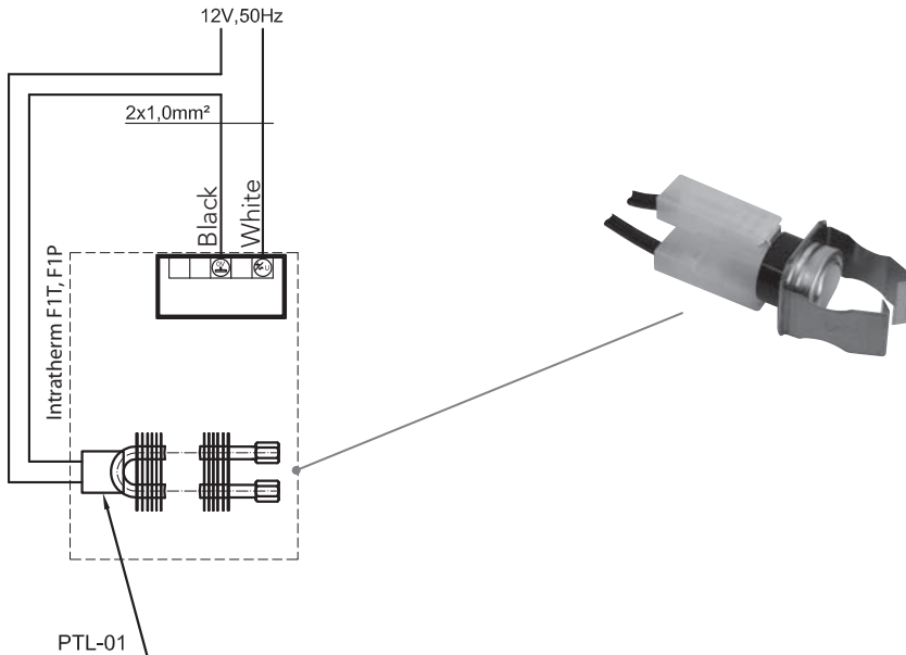
Block diagram no. 11 – Intratherm F1T, F1P with an assembly allowing for limited use of a PTL-01 fan
