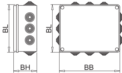
Surface-mounted version
