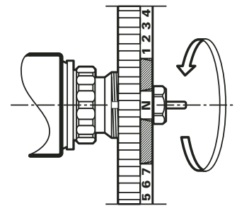
Detail Z
